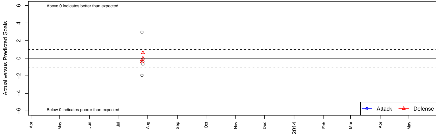
Maui Strikers B00 Dots are actual minus expected GF (blue circles) and GA (red triangles). Blue line is smoothed change in attack strength. Red is smoothed change in defense strength.
